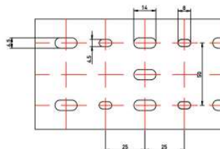
For Panel Trunking 75 x 75, 100 x 75 & 100 x 100
